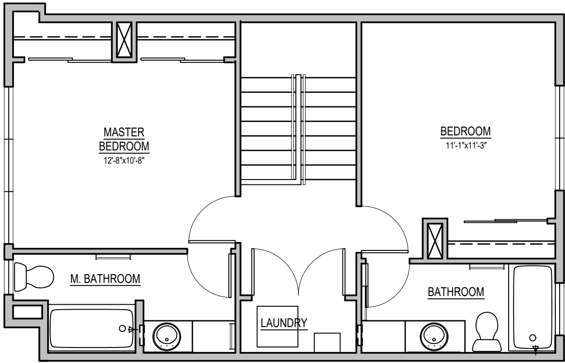
SECOND FLOOR
