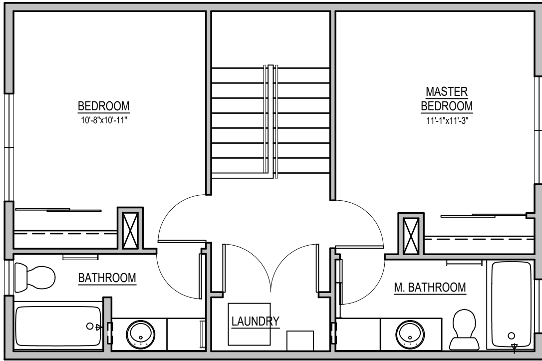
SECOND FLOOR
