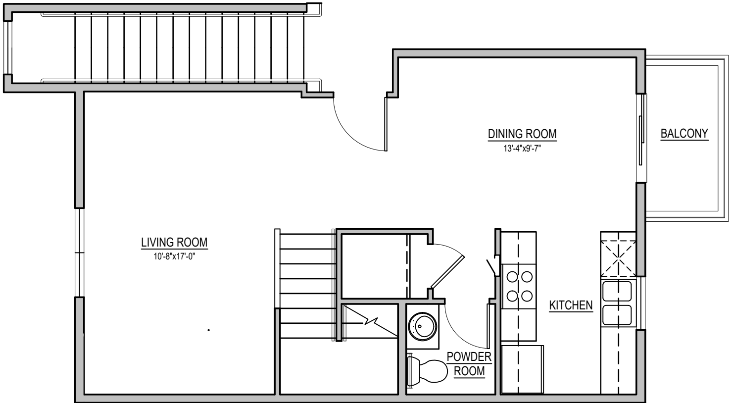
FIRST FLOOR
