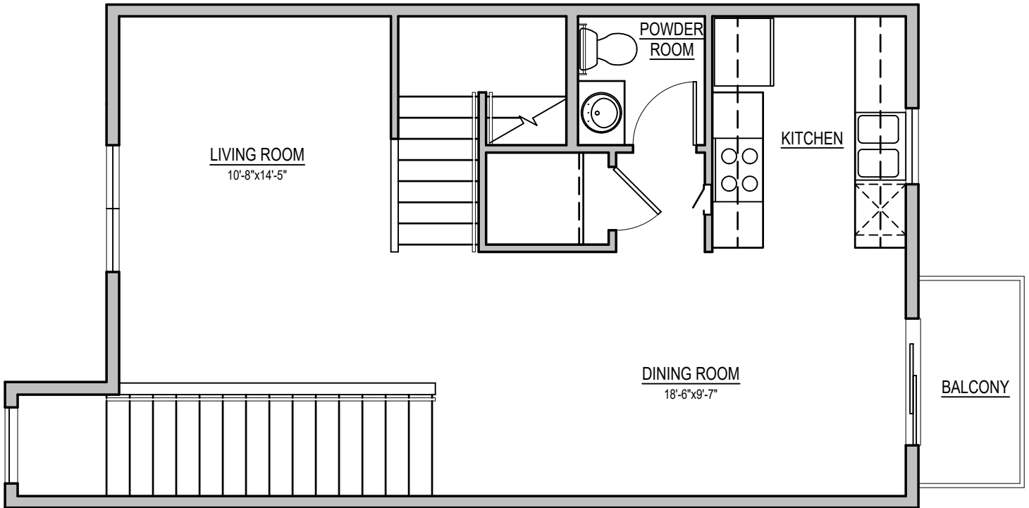
FIRST FLOOR
